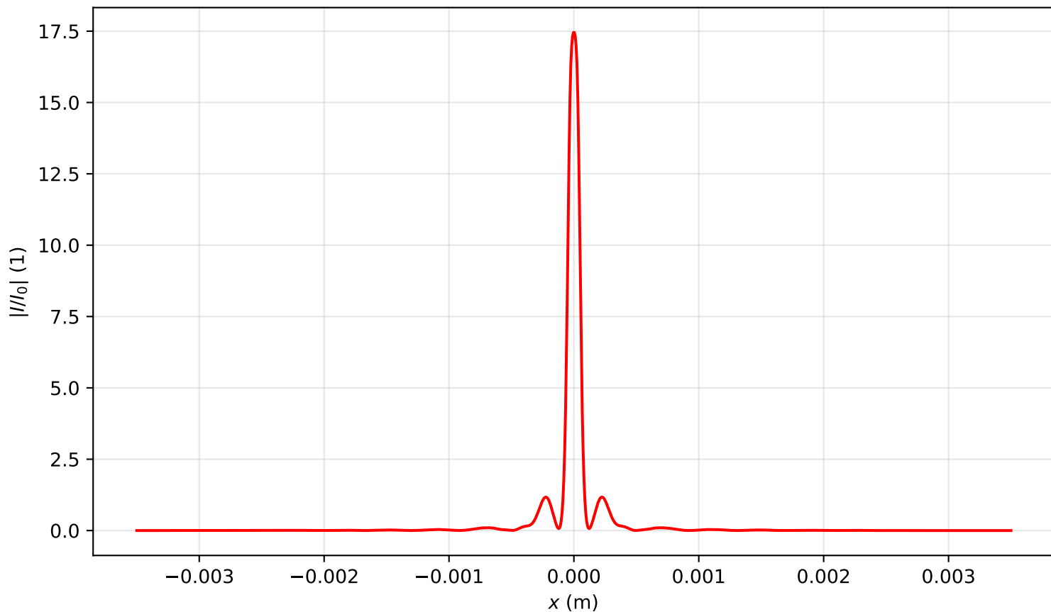
Intensity profile I(x, y = 0, z = 0.318)/I_0 , P_{in}=4.0P_{cr} , artificial time
